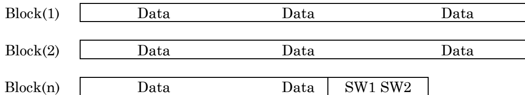
Figure 14: Chaining I-Blocks
