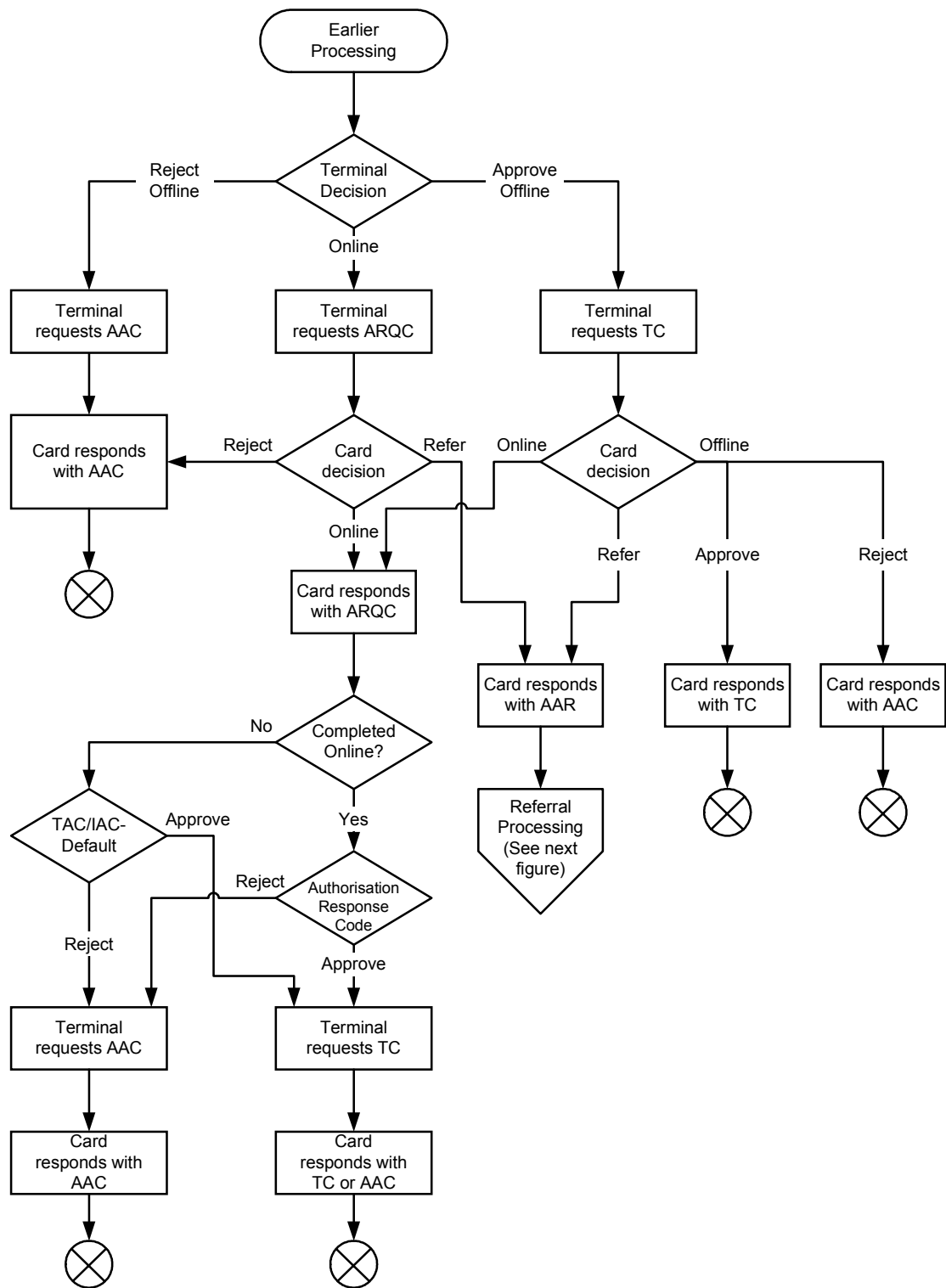
Figure 7: Use of GENERATE AC Options
