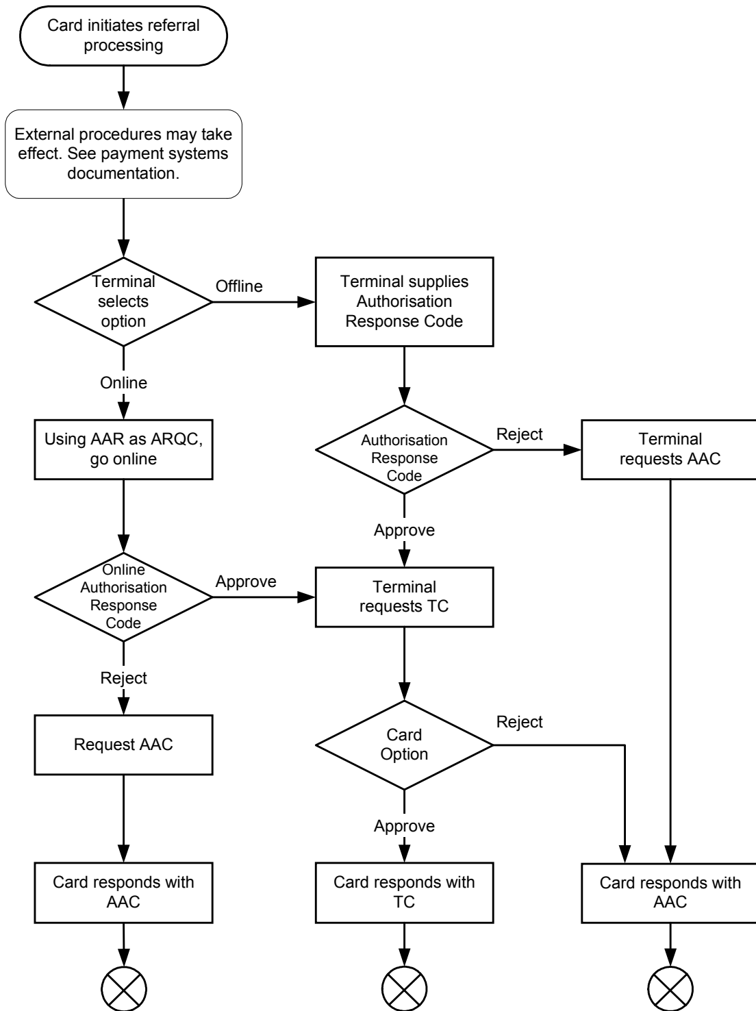
Figure 8: Use of GENERATE AC with Referrals
