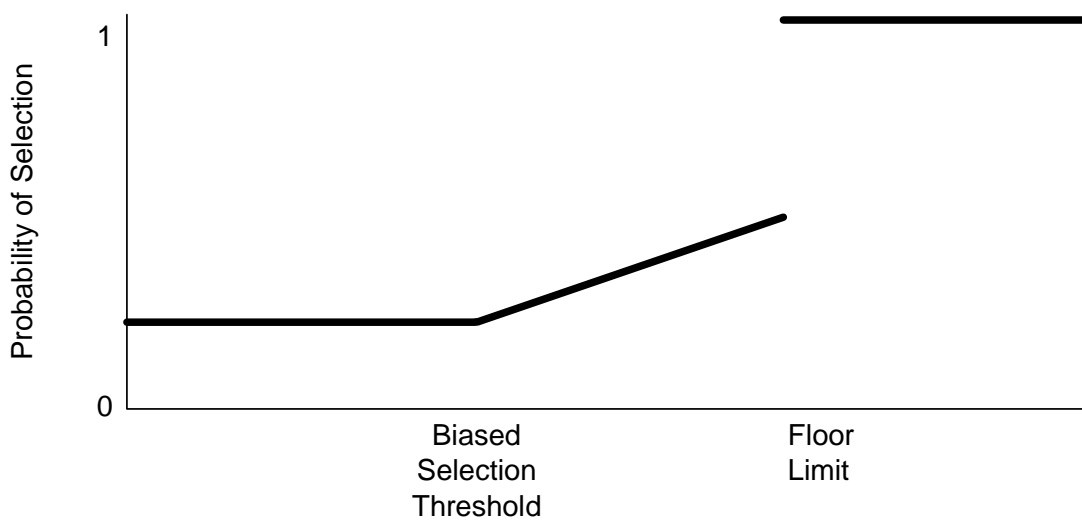
Figure 9: Random Transaction Selection Example
